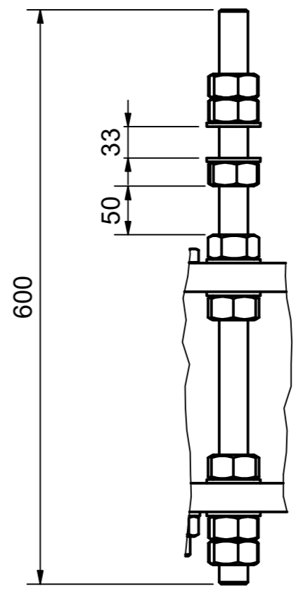
DETAIL A
