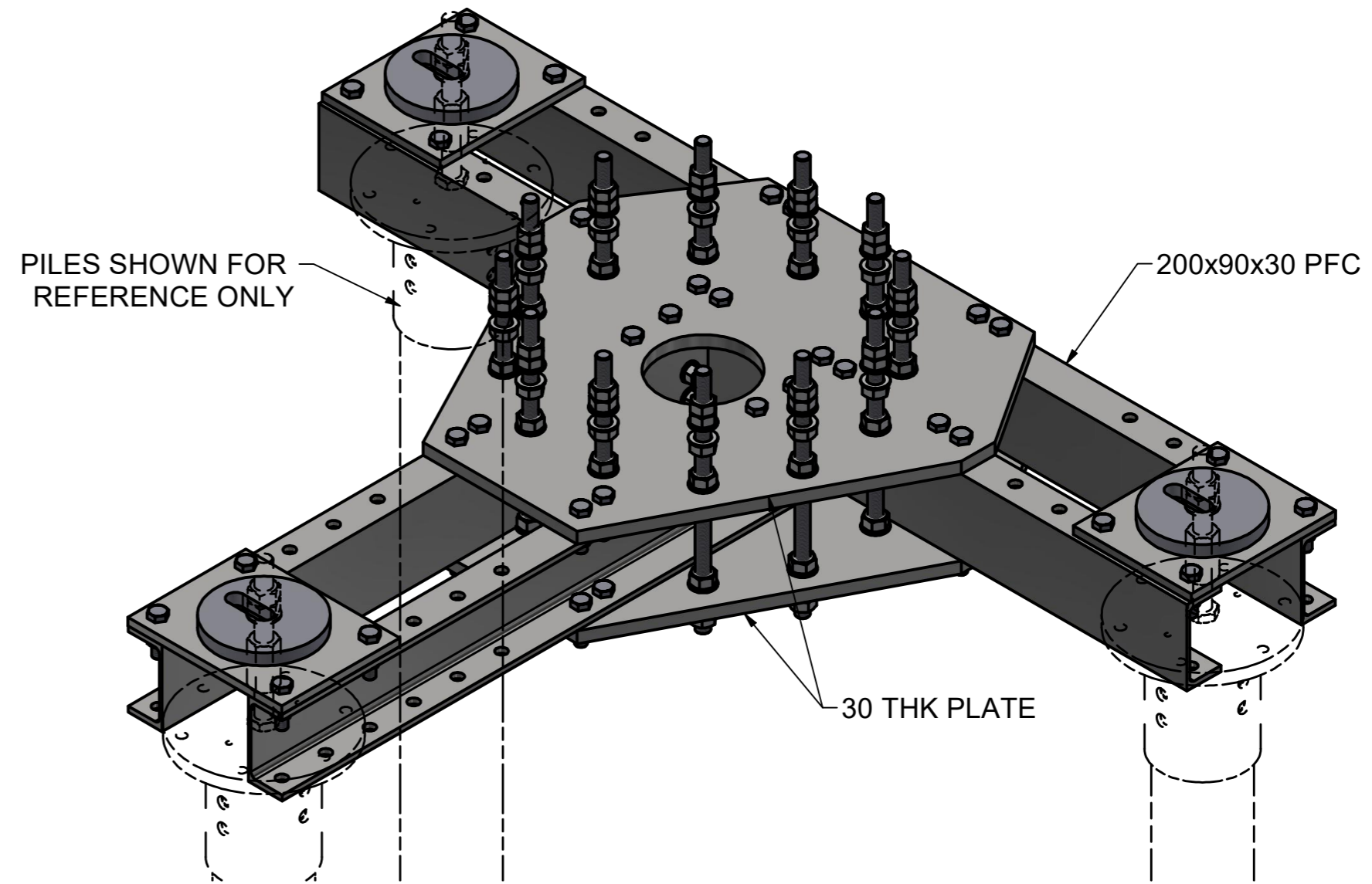
3D VIEW
